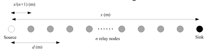
Fig. 4. WSN-HEAP in uniform string topology for railway track monitoring
