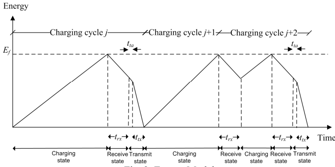
Fig. 2. Energy Model
