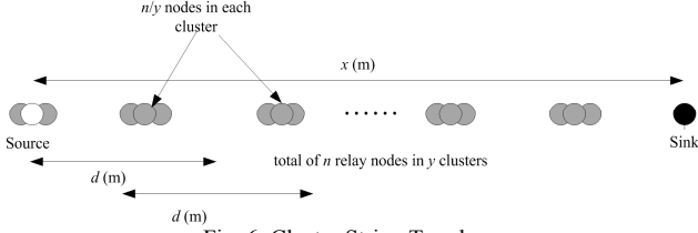
Fig. 6. Cluster String Topology
