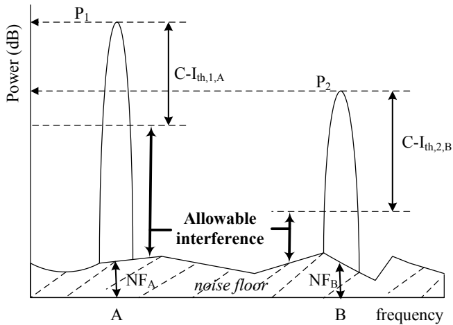
Fig. 2. An interference temperature model to determine the additional allowable co-channel interference to enable additional communication without degrading ongoing communication. This is given by P_i - C - I_{th,i,c} - NF_c , where P_i is the received power of the ongoing transmission from user i in channel c , NF_c is the noise floor and C - I_{th,i,c} is the carrier-to-interference ratio threshold for admissible call quality.
