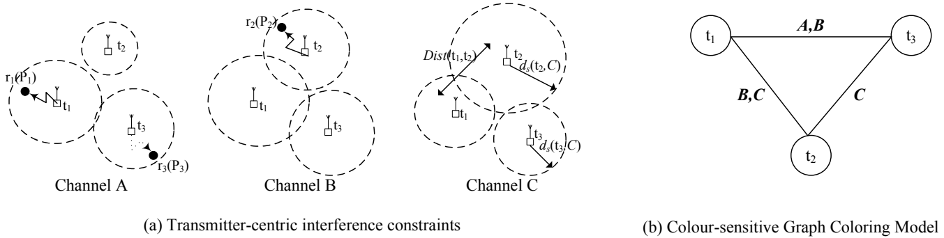
Fig. 1. (a) An illustration of binary and transmitter-centric interference constraints and (b) the corresponding colour-sensitive graph colouring model for allocating 3 channels, \{A, B, C\} amongst 3 transmitting users, \{t_1, t_2, t_3\} (represented by vertices). Each dotted circle represents the interference range of a node and the label on edge i-j indicates spectrum unusable by nodes i and j simultaneously.
