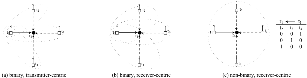
Fig. 3. Comparison of interference constraints for a multiple-interferer scenario: (a) Scope of binary transmitter-centric constraints (b) Scope of binary receiver-centric constraints and (c) Scope of non-binary receiver-centric constraints and an example of a relation comprising three tuples (right).
